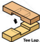
Tee Lap Joint
