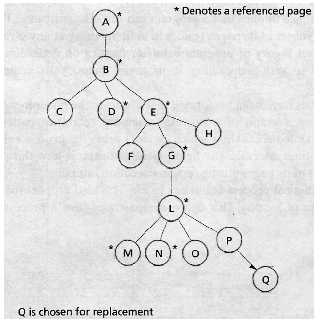
Figure 11.6 | Far page-replacement-strategy access graph.
