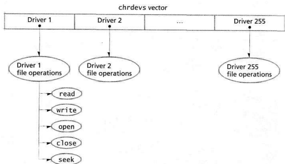
Figure 20.21 | chrdevs vector.
