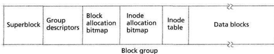
Figure 20.15 | Block group.
