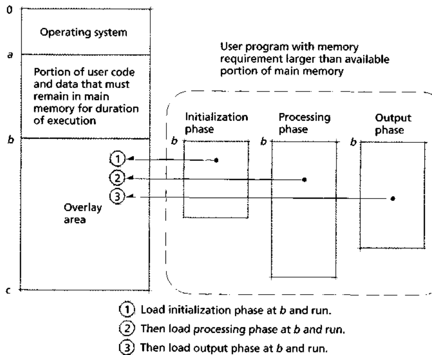
Figure 9.4 | Overlay structure.
