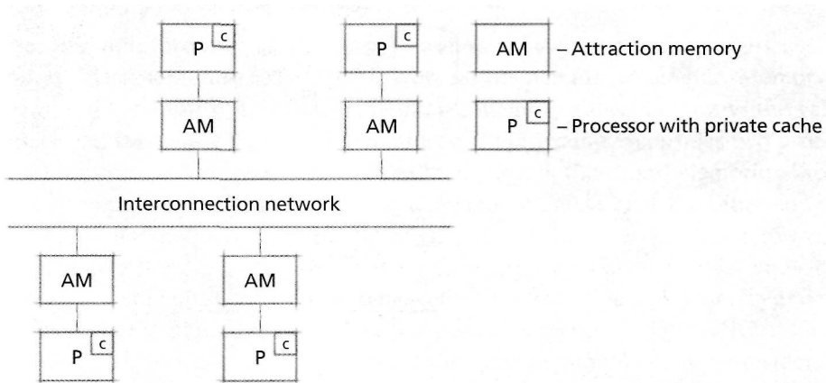
Figure 15.11 | COMA multiprocessor.
