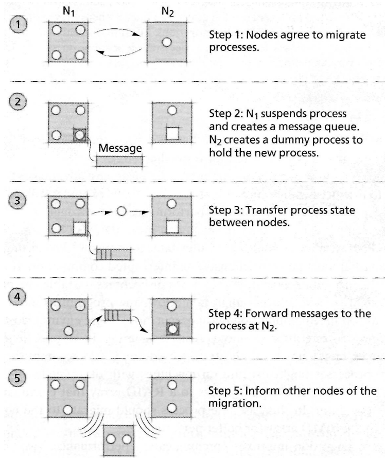
Figure 15.15 | Process migration.
