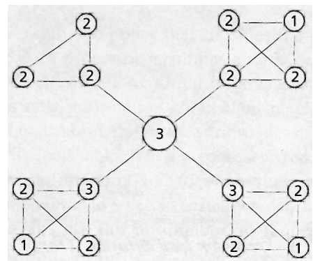
Figure 15.17 | Processor load diffusion. (Part 2 of 2.)
