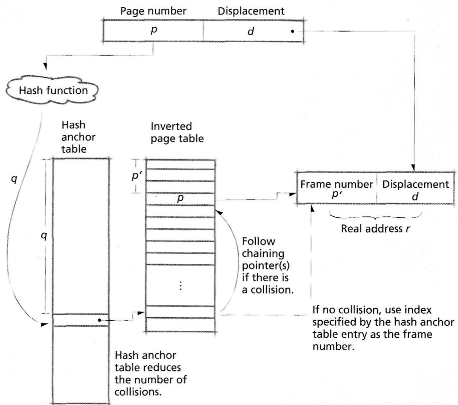
Figure 10.17 | Inverted page table using a hash anchor table.
