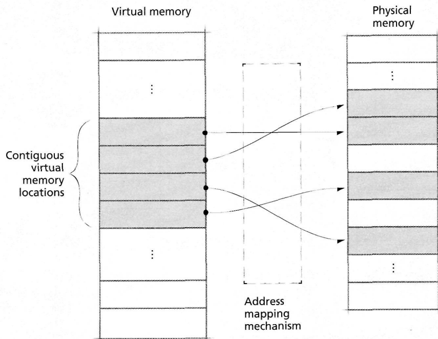
Figure 10.5 | Artificial contiguity.
