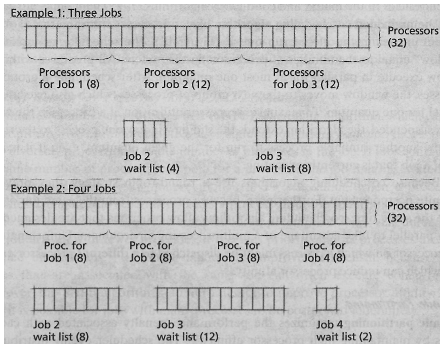
Figure 15.14 | Dynamic partitioning.
