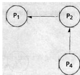
Figure 17.6 | System after deadlock has been eliminated.
