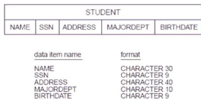
Figure 10.1 A record type STUDENT.
