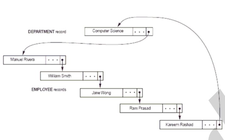
Figure 10.4 Alternate representation of a set instance as a linked list.
